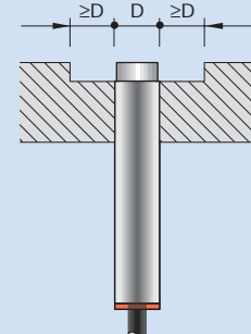
Flush mounting
